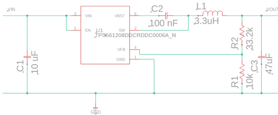
Figure 6.1B: Schematic of 3.3 Volt Regulator
