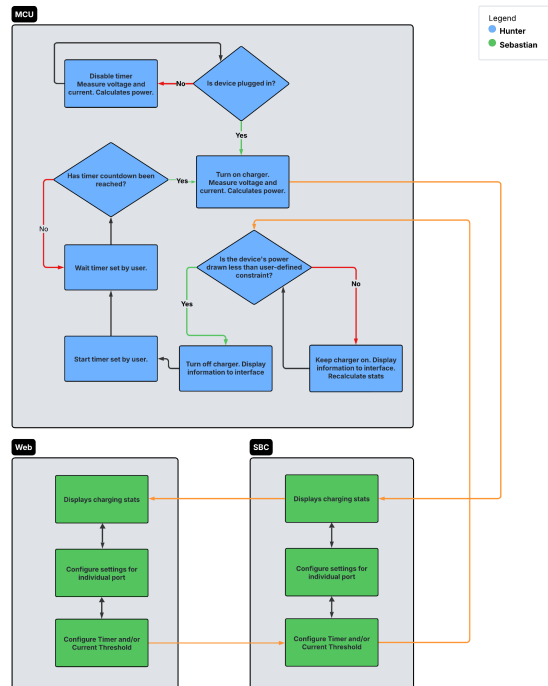
Figure 2.7: Software Block Diagram
