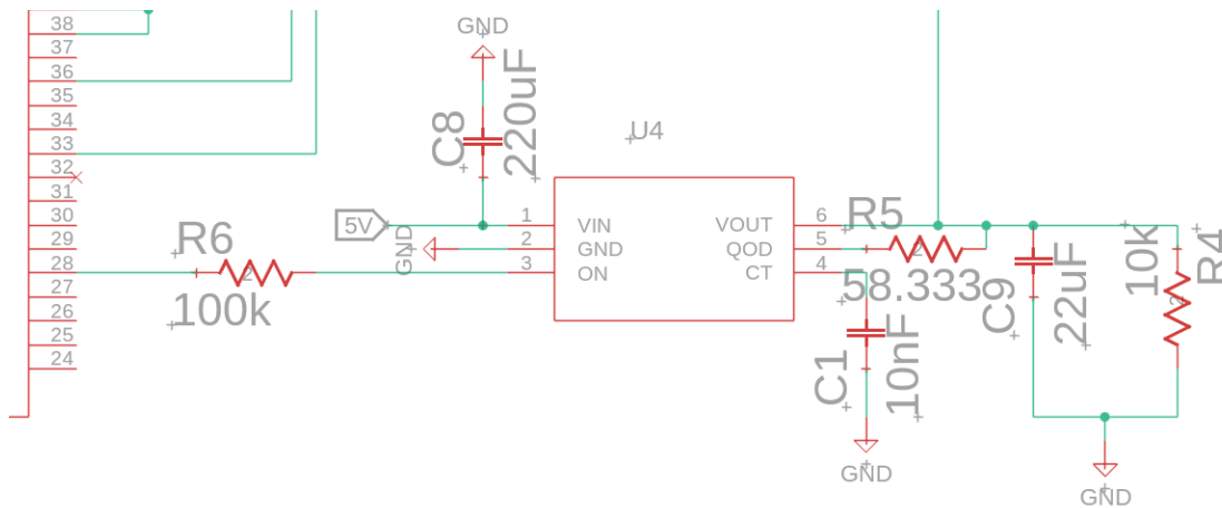
Figure 6.2A: Schematic of IC Load Switch
