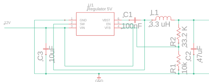
Figure 6.1A: Schematic of 5 Volt Regulator
