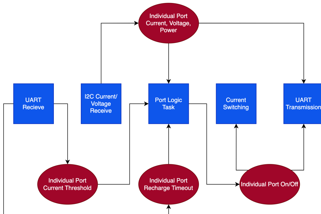
Figure 7.2b: MCU Shared Resource Diagram
