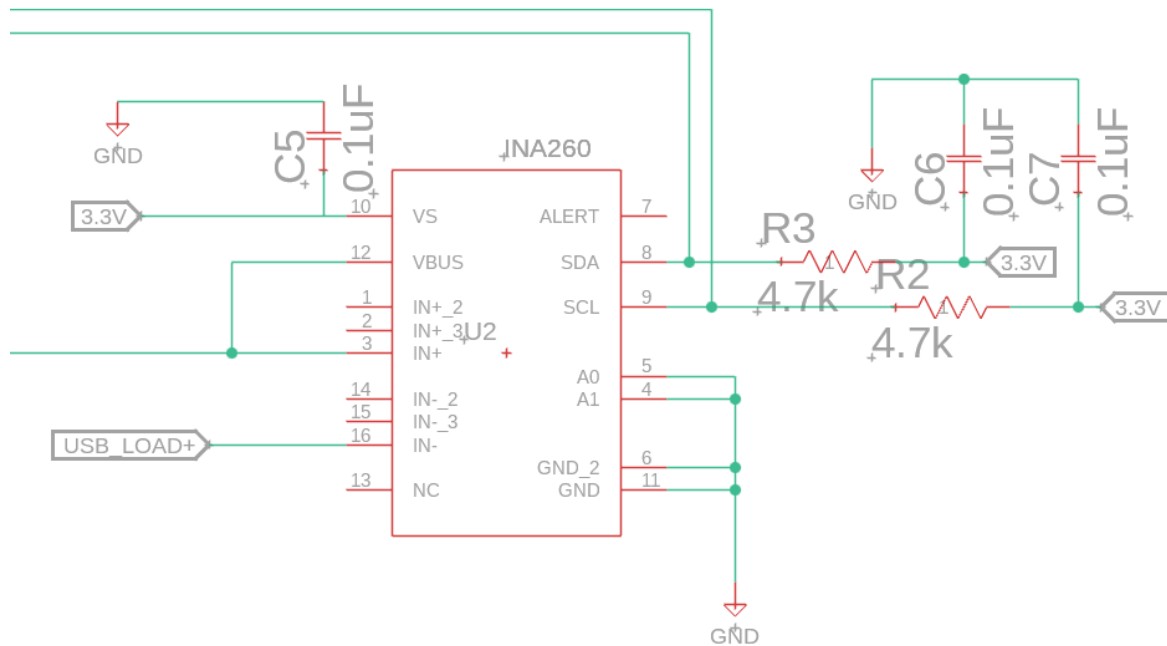
Figure 6.2B: Schematic of INA260 - Current and Voltage Measurement IC
