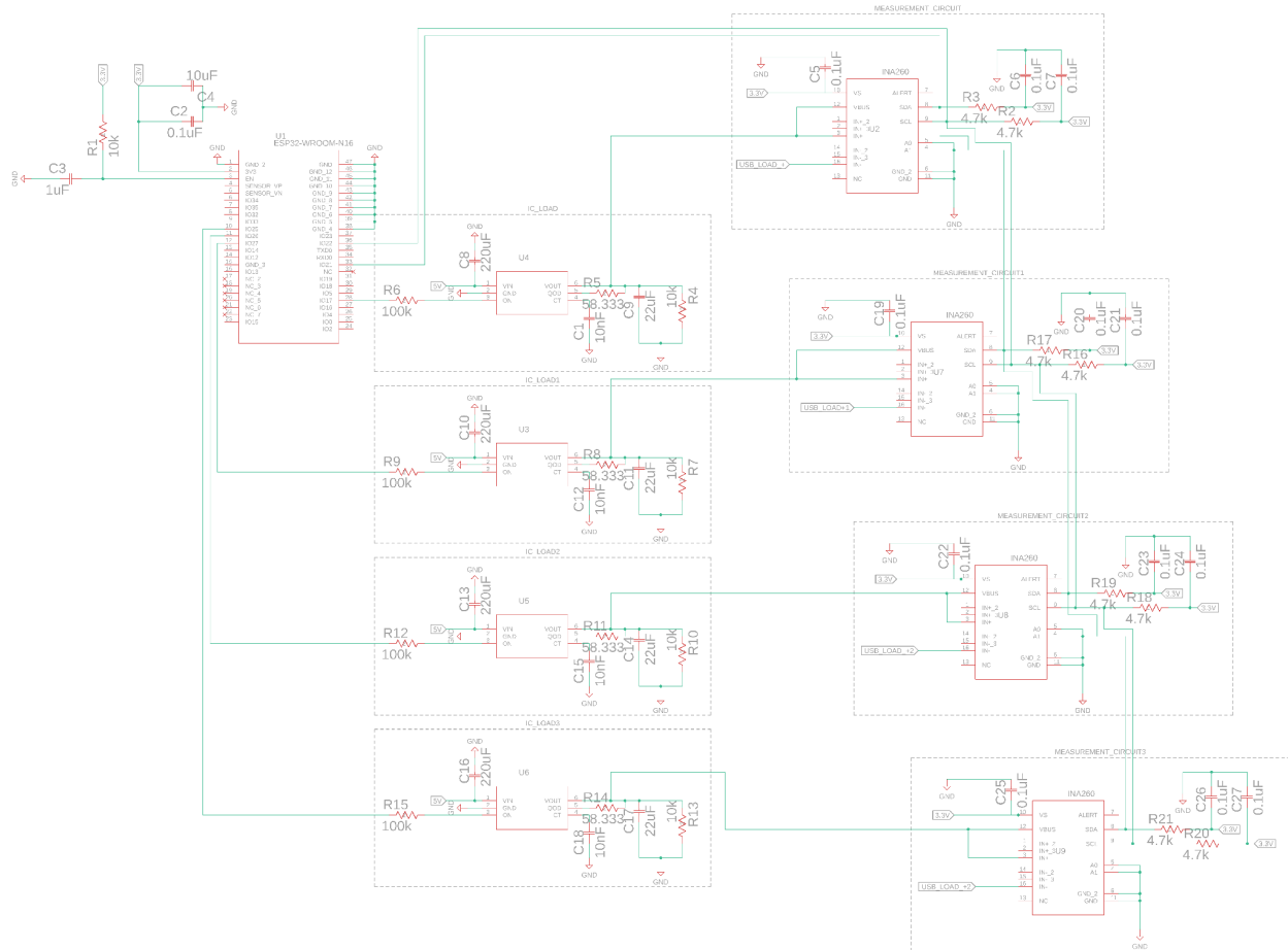
Figure 6.3A: Full Schematic of Charging Circuit - All 4 outputs
