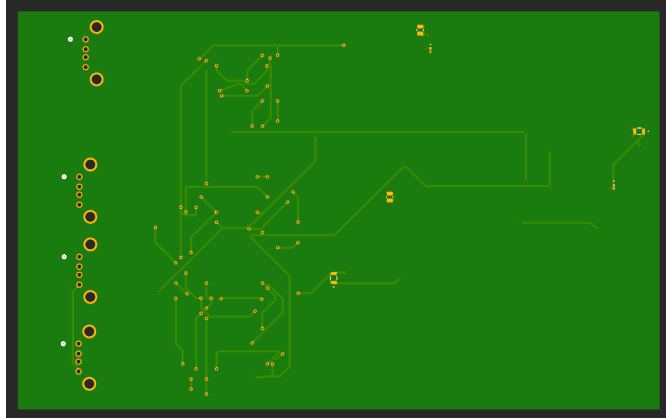
Figure 6.6D: PCB Preview of Main PCB - Bottom
