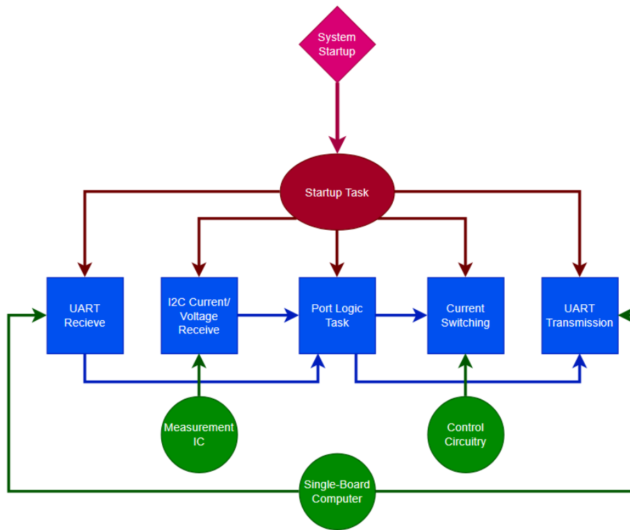
Figure 7.2a: MCU Task Block Diagram
