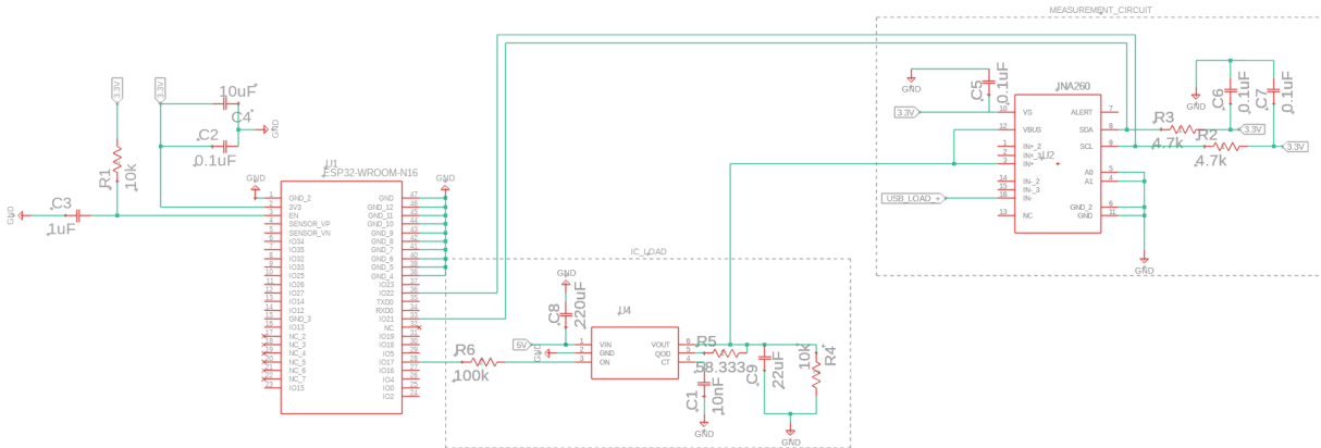
Figure 6.3B: Schematic of Charging Circuit - 1 Output.
