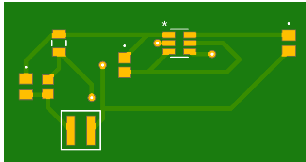
Figure 6.6A: PCB Preview of 5V regulator - Top
